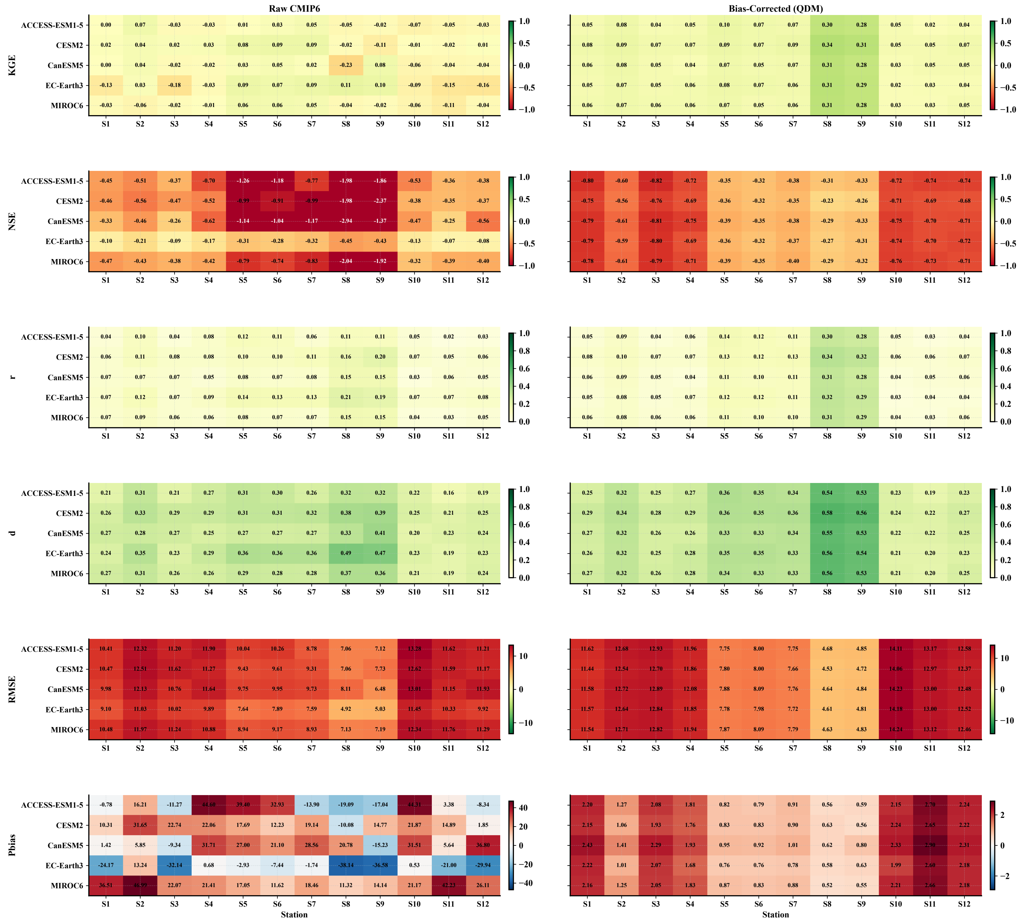
Model Performance Heatmap — Daily Scale Raw CMIP6 (left) vs Bias-Corrected QDM (right) | Obs: 1981–2014
